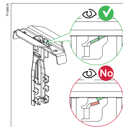
When the bracket needs to be reinstalled, correct the click lip to the initial position and make sure the click lip is locking properly.
