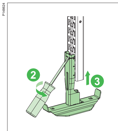
Use the screwdriver as a lever to 2 gently release the click lip from the rail. Then 3 push the adaptor up to release the L hooks from the rail.
