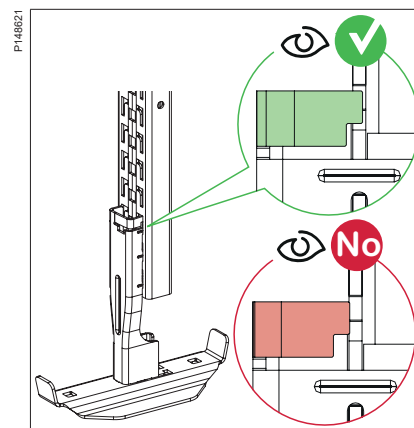
If the adapter needs to be reinstalled, correct the click lip to the initial position and make sure the click lip is locking properly.
